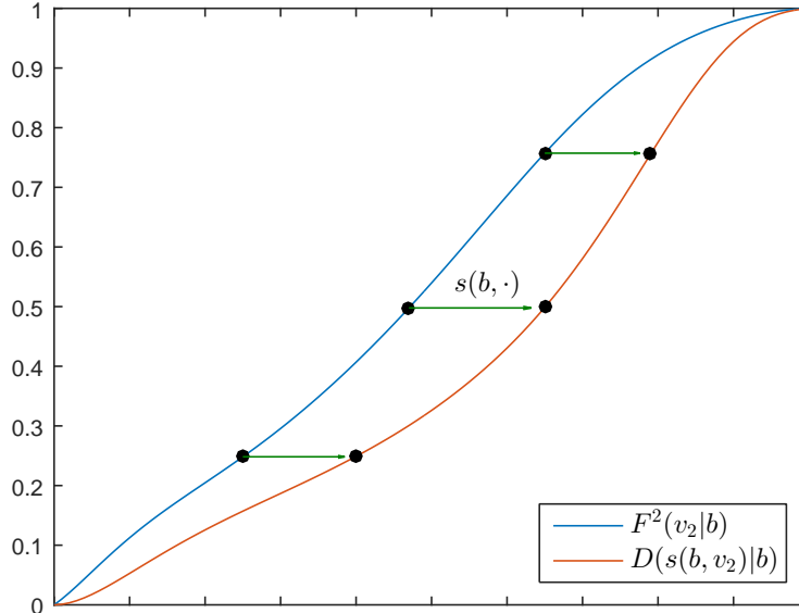
Figure 2: Nonparametric identification of s(b, \cdot)
